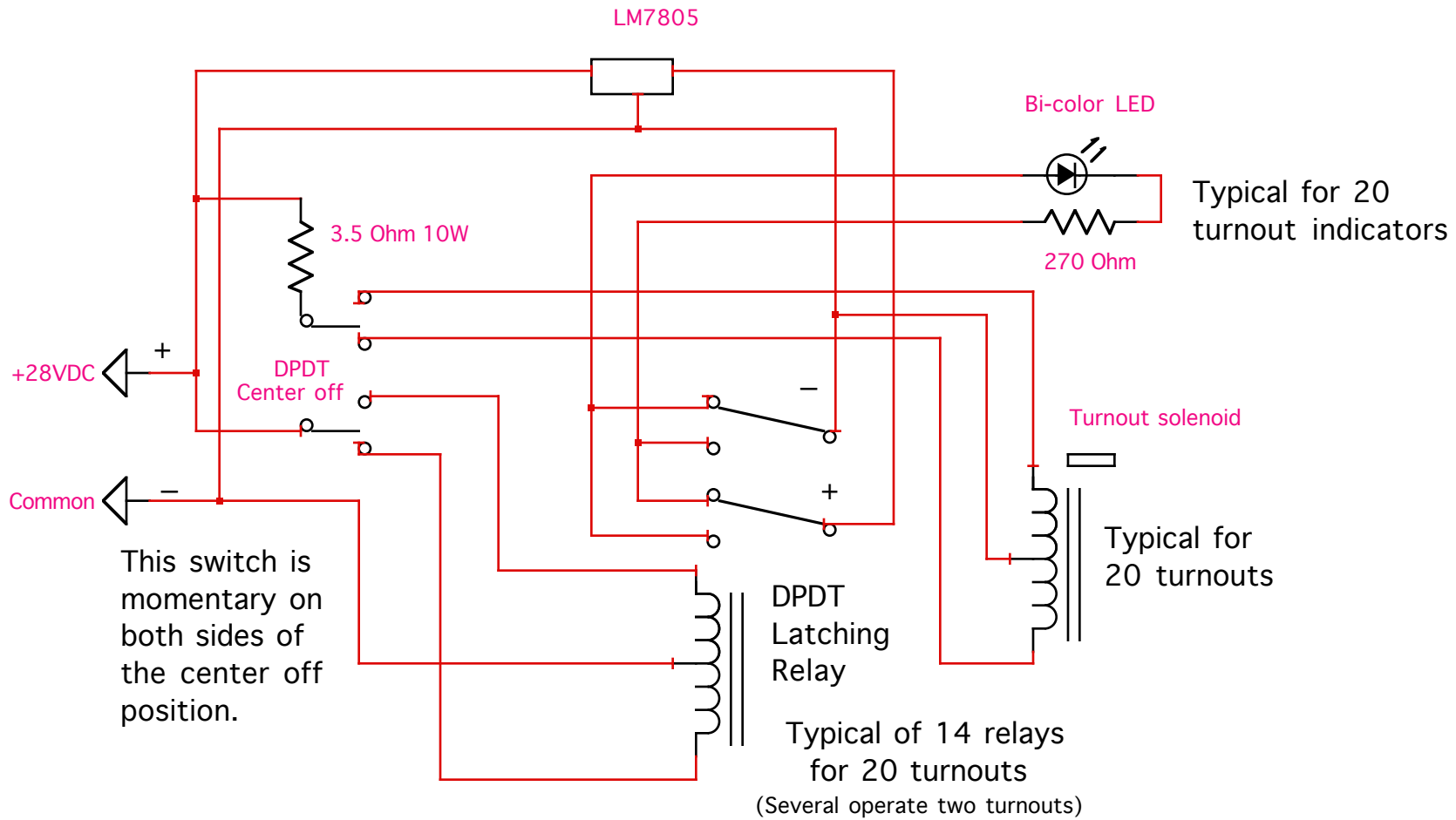
Model railroad turnout switch control with red/green LED indicators
